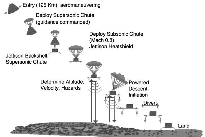
Fig. 1 MSL entry, descent, and landing sequence of events.
